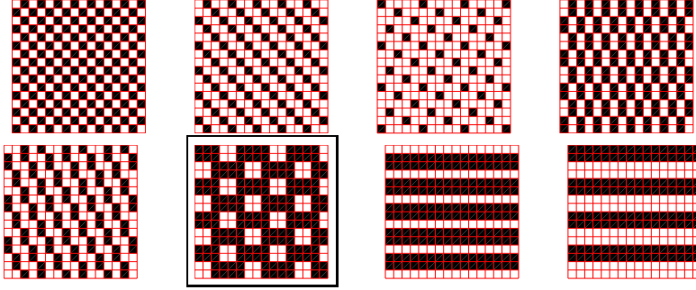
Figure 2.3: Isolated balanced two-colorings on square lattice with NN coupling. The pattern in the box is not a fixed-point subspace of a subgroup of \mathcal{G}_{\mathcal{L}} .
