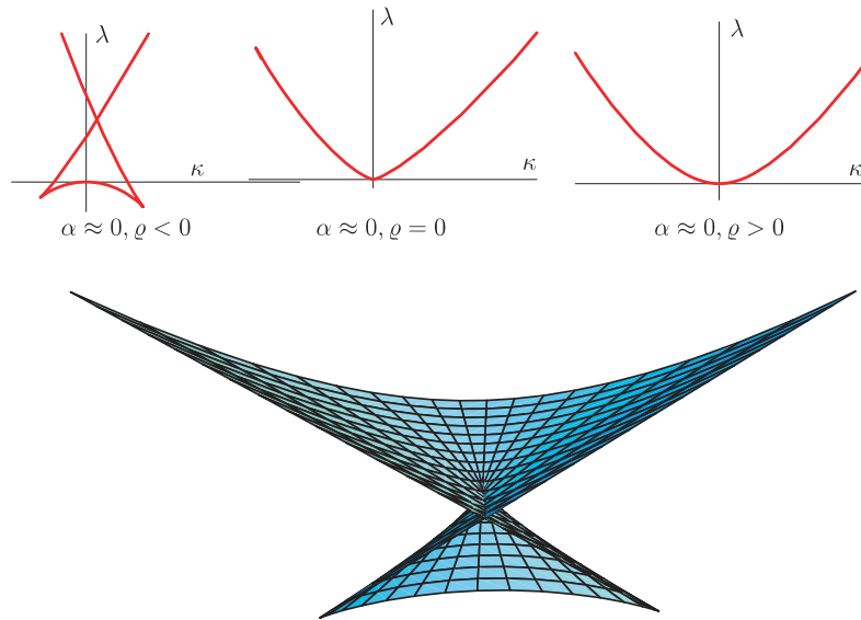
Figure 5. The discriminant set of the family \bar{Q}(u, \kappa, \lambda, \varrho, \alpha) = u^4 - u^5 + 2\alpha u^3 + \varrho u^2 + \lambda u + \kappa parametrized by (5.13), locally near 0 \in \mathbf{R}^4 . This surface is the product of the real line and a swallowtail, near 0 \in \mathbf{R}^4 . Top row: cross-sections of D_{\bar{Q}} with planes (w, \alpha) = (w_0, \alpha_0) . Bottom row: cross-sections of D_{\bar{Q}} with hyperplanes \alpha = \alpha_0 .
